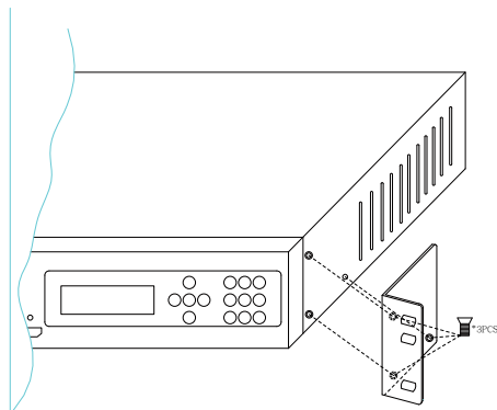
Figure 1. Rack-Mount Installation
